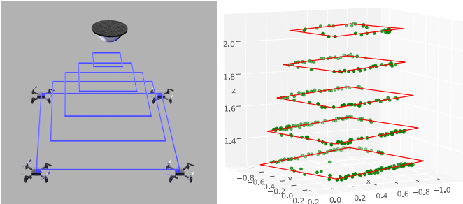
Fig. 5. Left: CAD Model depicting the setup for metaveillance of a surveillance camera. Right: Computerized 3D model of veillance flux.
