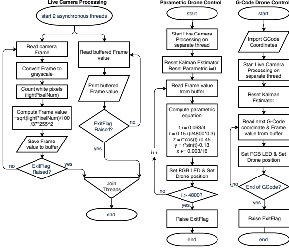
Fig. 4. Flowcharts for the Live Camera Processing, Parametric Drone Control, and G-Code Drone Control routines
