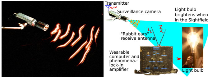
Fig. 1. Mann's metaveillance apparatus from the mid 1970s [15], [16], [17] used one or more light bulbs fed from a wearable computer and lock-in amplifier designed to lock in on television signals from surveillance cameras. The light bulb transitions from a dim red glow to a brilliant white whenever it enters the camera's field-of-view, and then the bulb brightness drops off again when it exits the camera's field of view. Waving it back and forth in a dark room reveals to the human eye, as well as to photographic film (picture at left) the camera's capacity to "see".
